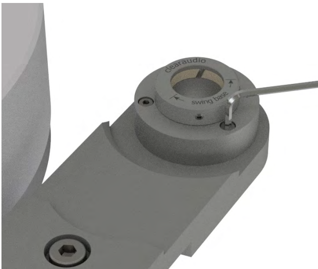
Pic. 5a: Installation of the swing base
