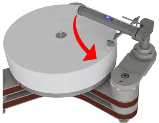
Pic. 5b: swing direction of the tonearm
