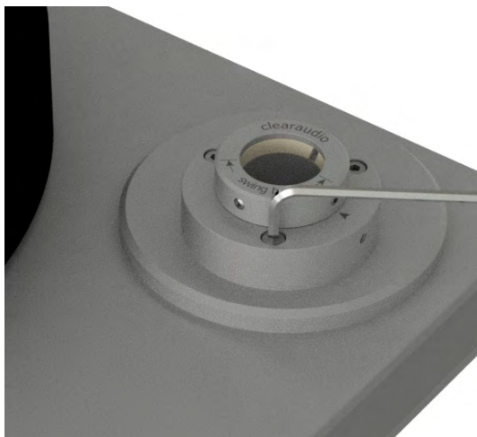
Pic. 3a: Installation of the swing base
