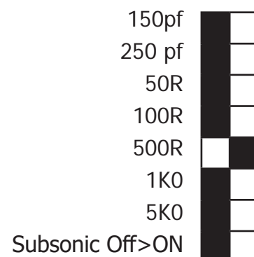
Pic. 2.3: Adjustment 500 Ohm
