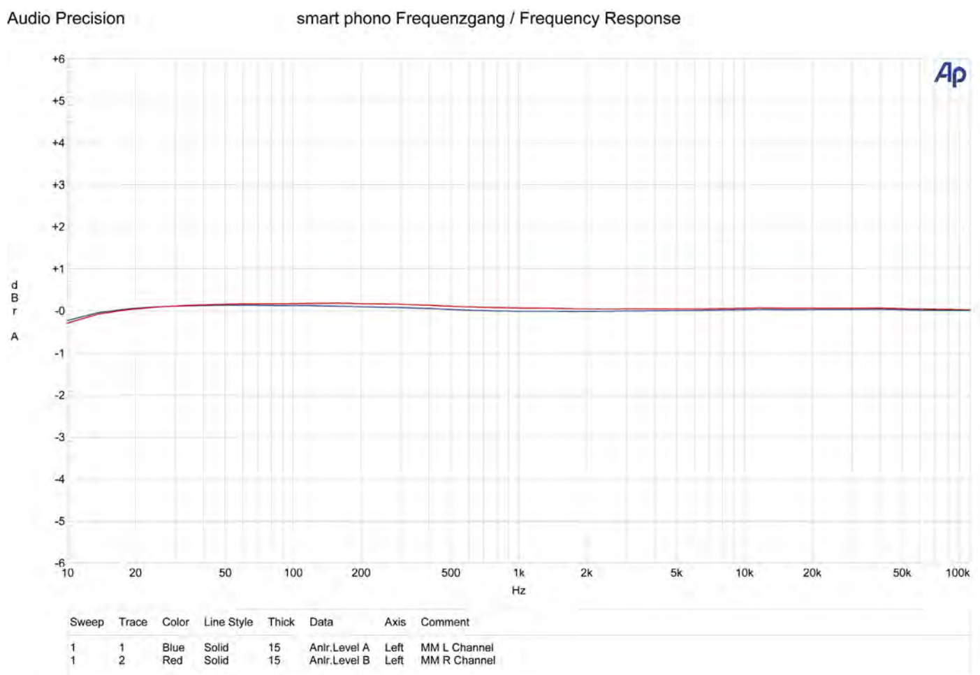
Pic. 5: Frequency Response
