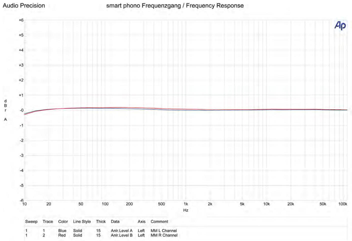
Abb. 5: Frequenzgang
