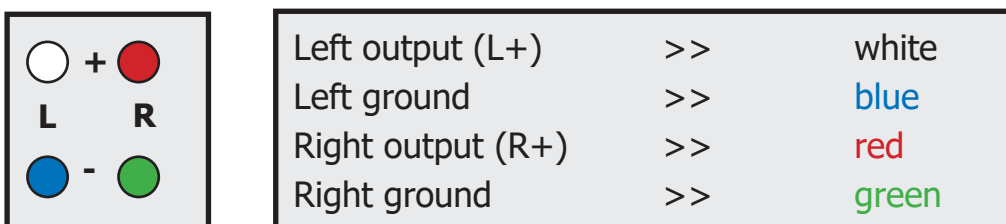
Pic. 1: Color marking of the signalpins
