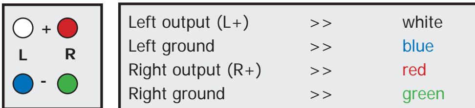
Pic. 1: Color marking of the signalpins
