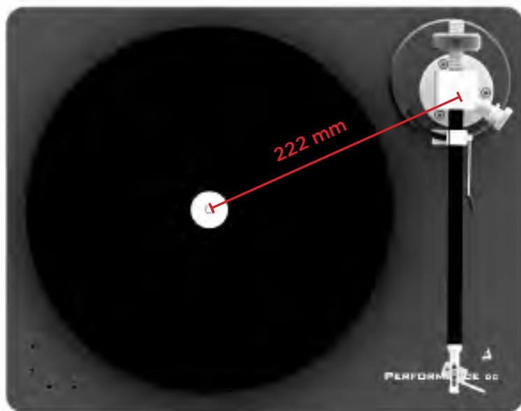
Pic. 6: Distance from pivot to stylus
