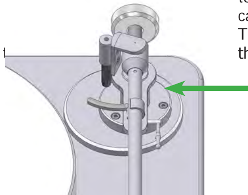
Pic. 7: Adjustment of the tonearm height
